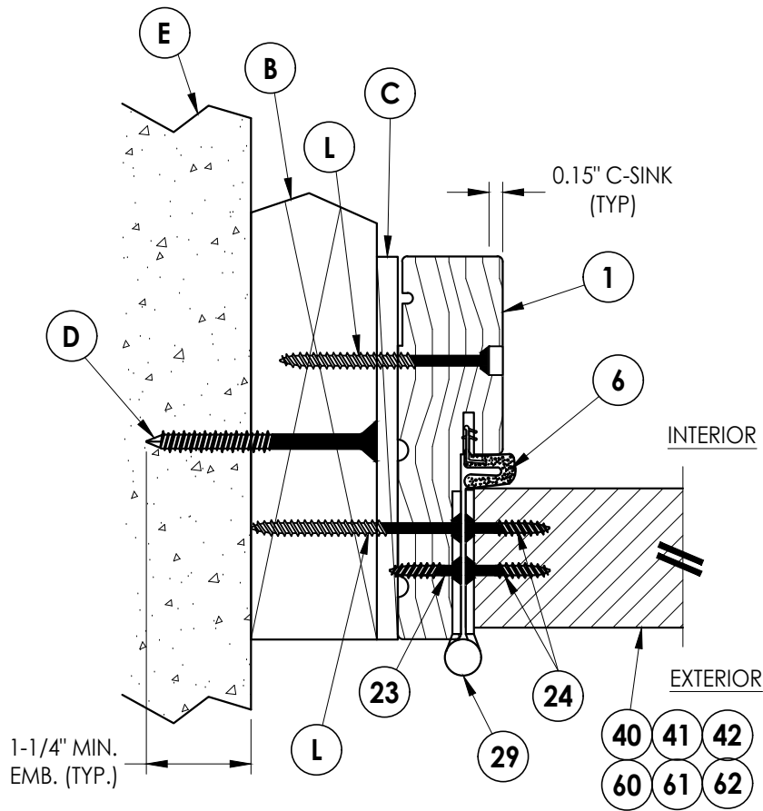
2 5 HORIZONTAL CROSS SECTION Shown w/ 2X Buck Outswing shown (Inswing similar)
